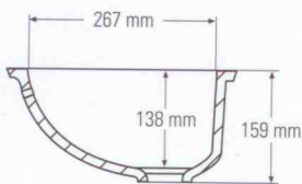
Side cross-section
