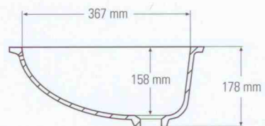
Side cross-section
